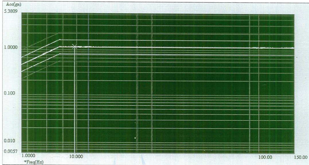
Sine vibration test profile
