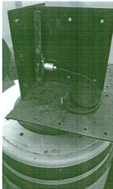
Test set up Z-Axis
